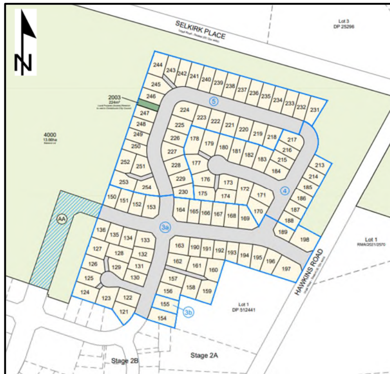
Figure 1: Extract from the Oakbridge Scheme Plan – Stages 3-5 (overall plan) (DWG 350/D). Not to scale.
